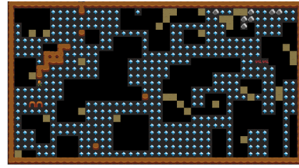
(b) paretoMCTS
