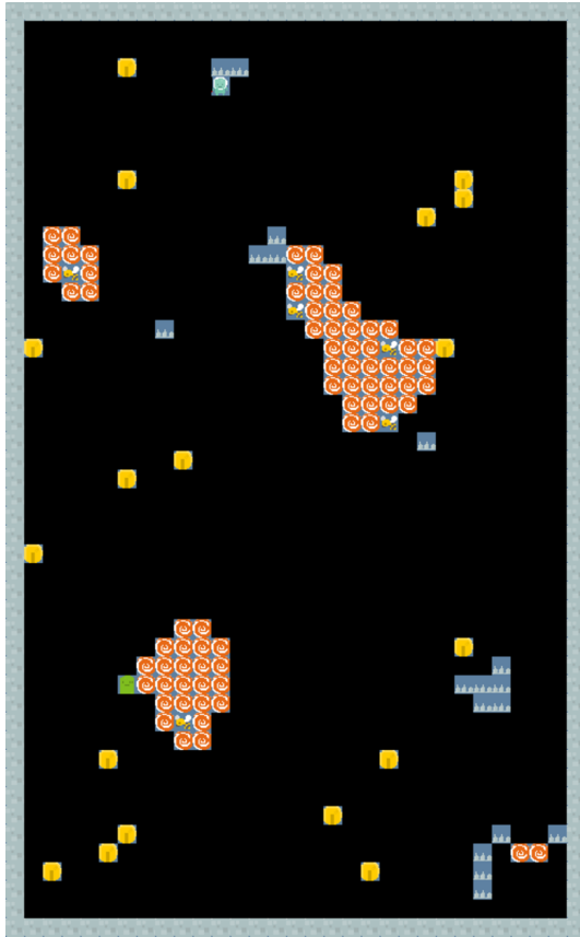
(c) paretoMCTS
