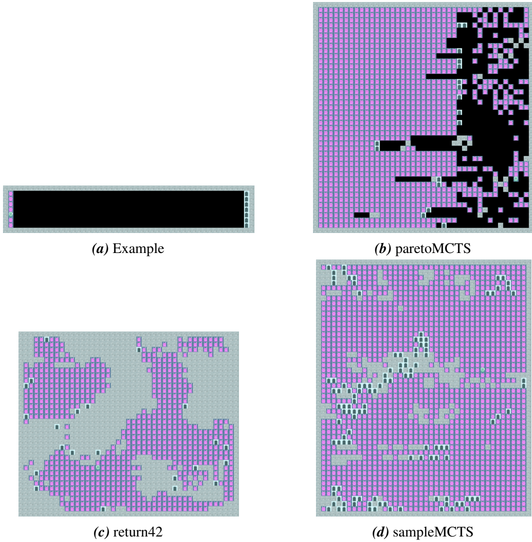
Figure A.22.: Generated levels for the game Camel Race and one human-made example level design for comparison.
