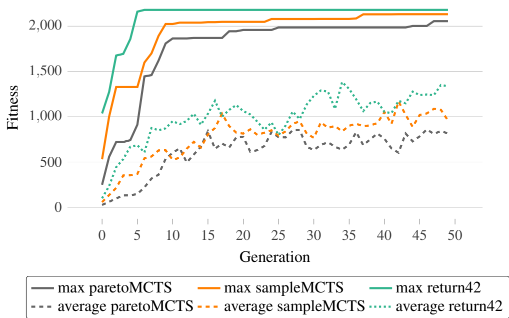
Figure A.33.: Average and maximum fitness values for the game Pacman for all 50 generations using three different agents for the simulation.
