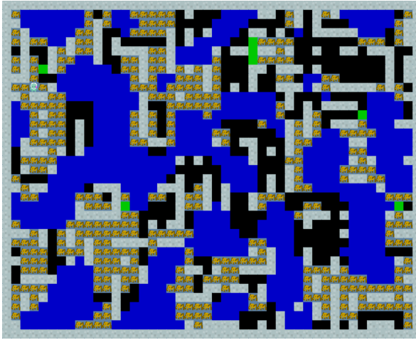
(c) return42
