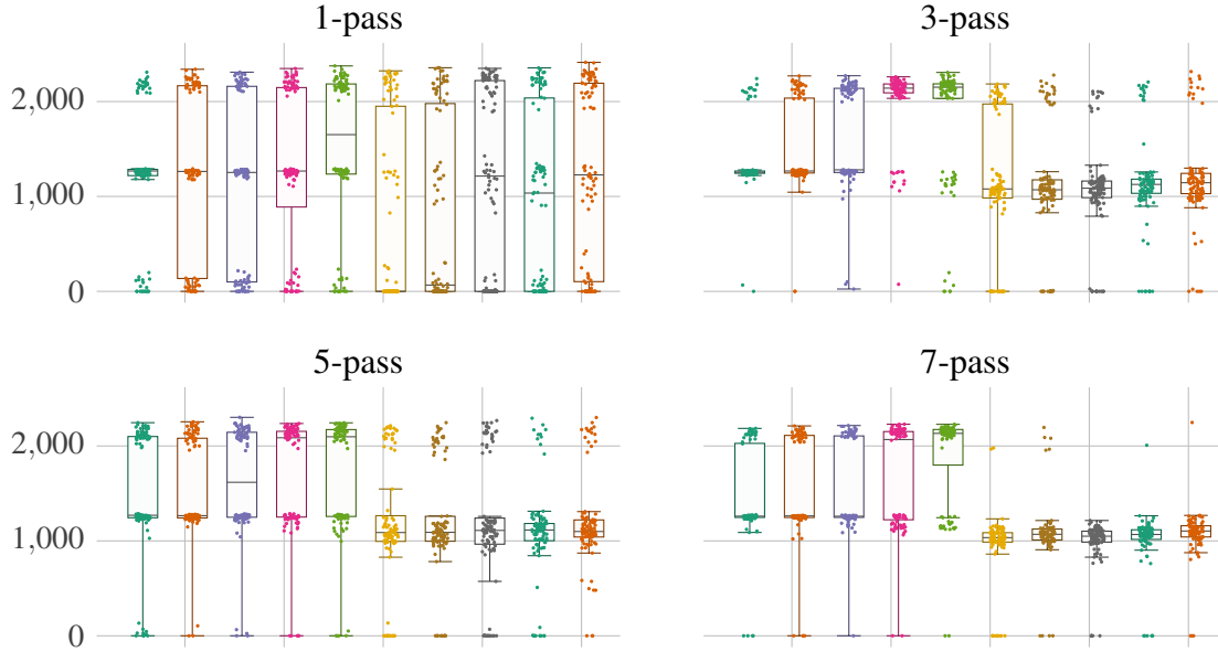
Figure 5.2.: Plotted fitness values of ten different individuals that played the game aliens 100 times with 1,3,5 and 7 simulation passes.
